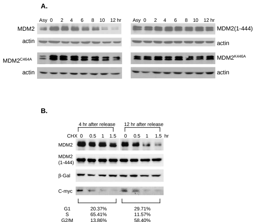
Fig. 2. The RING finger domain of MDM2 is required for cell cycle-dependent regulation. A: HeLa cells were transfected with pCMV-MDM2, pCMV-MDM2(1–444), pCMV-MDM2 C464A or pCMV-MDM2 K446A . 6 h after transfection, cells were trypsinized and reseeded for 4 h. Cells were then synchronized by double thymidine block and release. Equal amounts of total proteins were separated on 10% SDS-PAGE and subjected to Western blot analysis for MDM2 or actin. B: MDM2 protein is stabilized at S phase. U2-OS cells were transfected with pCMV-β-Gal and pCMV-MDM2 or pCMV-MDM2(1–444). 6 h after transfection, cells were synchronized by double thymidine block and were then treated with cycloheximide (CHX) at either 4 h or 12 h after release of thymidine treatment. Cells were collected at the indicated time points. Aliquots of cells were subjected to FACS analysis, whereas equal amounts of total proteins derived from the cell lysates were separated on 10% SDS-PAGE and subjected to Western blot analysis for MDM2, β-galactosidase and C-Myc.
